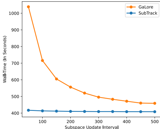
Figure 1: Comparing runtimes of GaLore and SubTrack. RoBERTa-Base is fine-tuned for 10 epochs on COLA task for different subspace update intervals. Notice that by increasing this number, the update frequency actually decreases, as it indicates the number of iterations between two subspace update steps.
